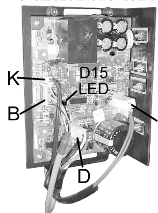
910E/920E lower board
